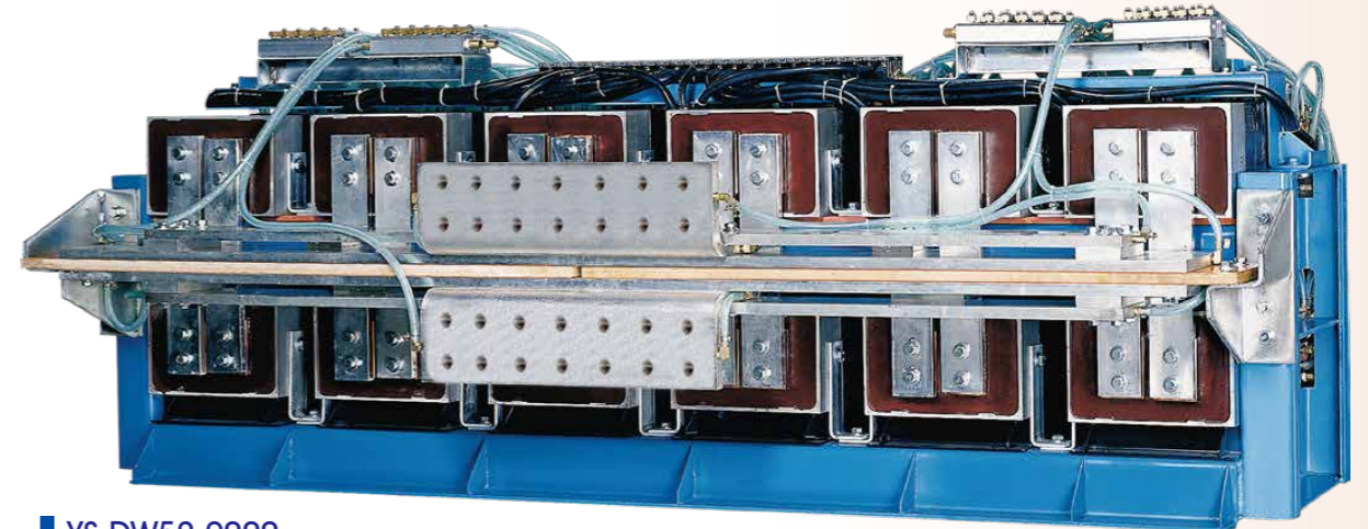
YS-DW52-9000 背式整流型熔接變壓器 DC Welding Transformer(Back-end) 柵板焊接機械專用 Grating Welding Machines-use 900KVA三相入力 Three phase input
