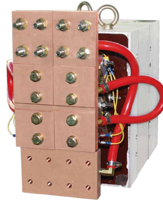
YS-DWH2-1500102 變頻式直流熔接變壓器 Inverter Welding Transformer 150KVA 1200Hz
