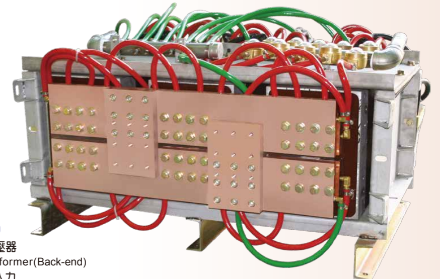
YS-DW52-9000 背式整流型熔接變壓器 DC Welding Transformer(Back-end) 柵板焊接機械專用 Grating Welding Machines-use 900KVA三相入力 Three phase input
