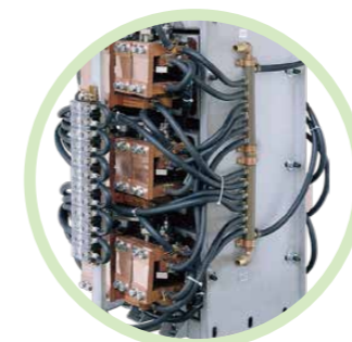
電源端子及冷卻水管集中裝置 Power Terminal and Cooling Water Collector
