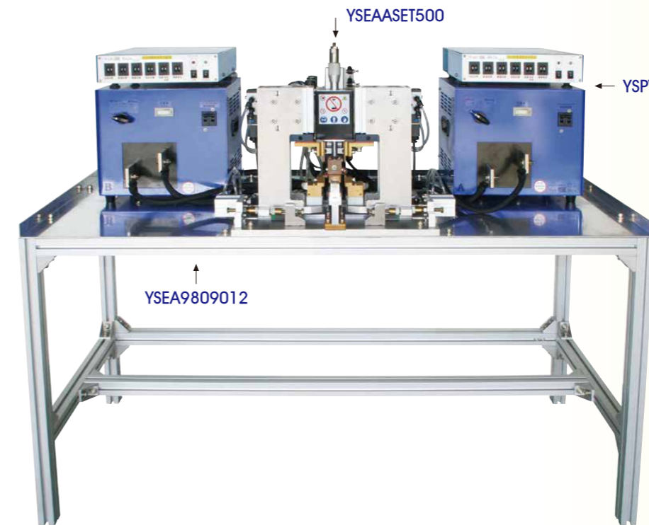
YS-CB00055201 (YSPW3100055 + YSEAASET500 + YSEA9809012) 5.5KVA空壓式碰焊機-雙機頭 Pneumatic Butt Welding Machine- Twin-Head
