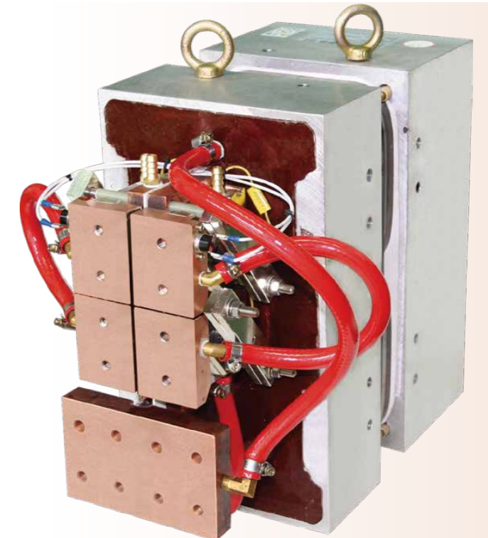
YS-DWH2-1500103 變頻式直流熔接變壓器(輪焊用) Inverter Welding Transformer (For SEAM welder use) 150KVA 1200Hz
