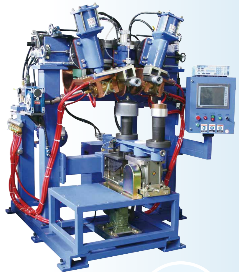
YS-CW250 250KVA雙頭輪焊機 Twin-Head Type Seam Welders
