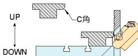
T型工件倒角 T type workpiece chamfering
